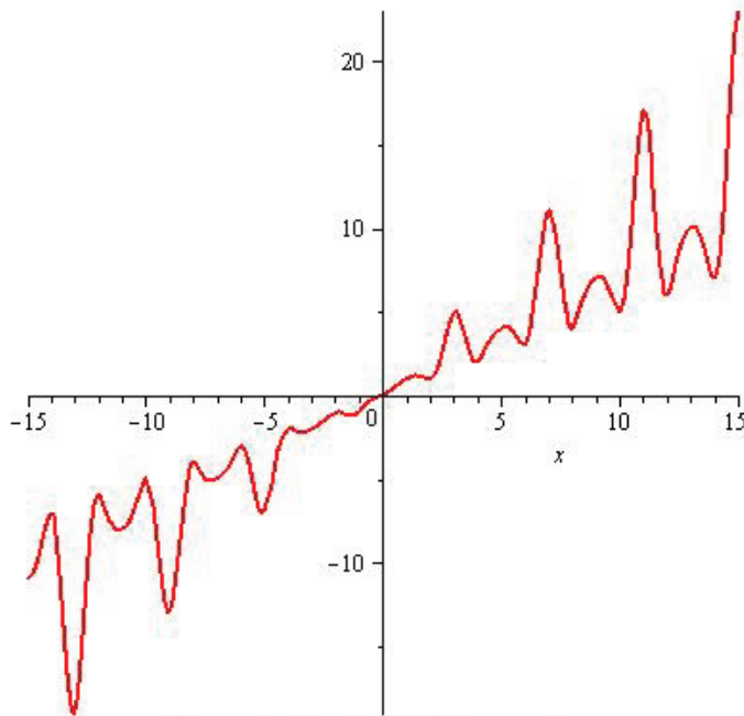
Figure 1: Graph of F^*(z) on reals
