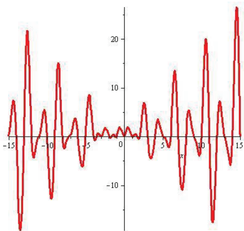
Figure 2 : Graph of F^{*'}(z) on reals
