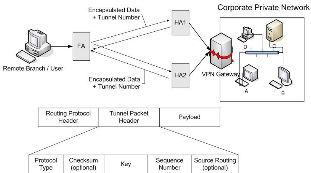
Figure 5: Multiple VPN tunnels illustration
