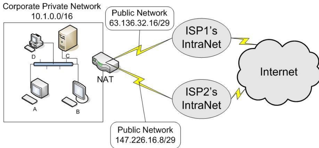
Figure 4: Multi-homing with NAT support
