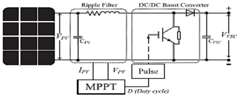
Figure 4: Controller mechanism of the boost converter.
