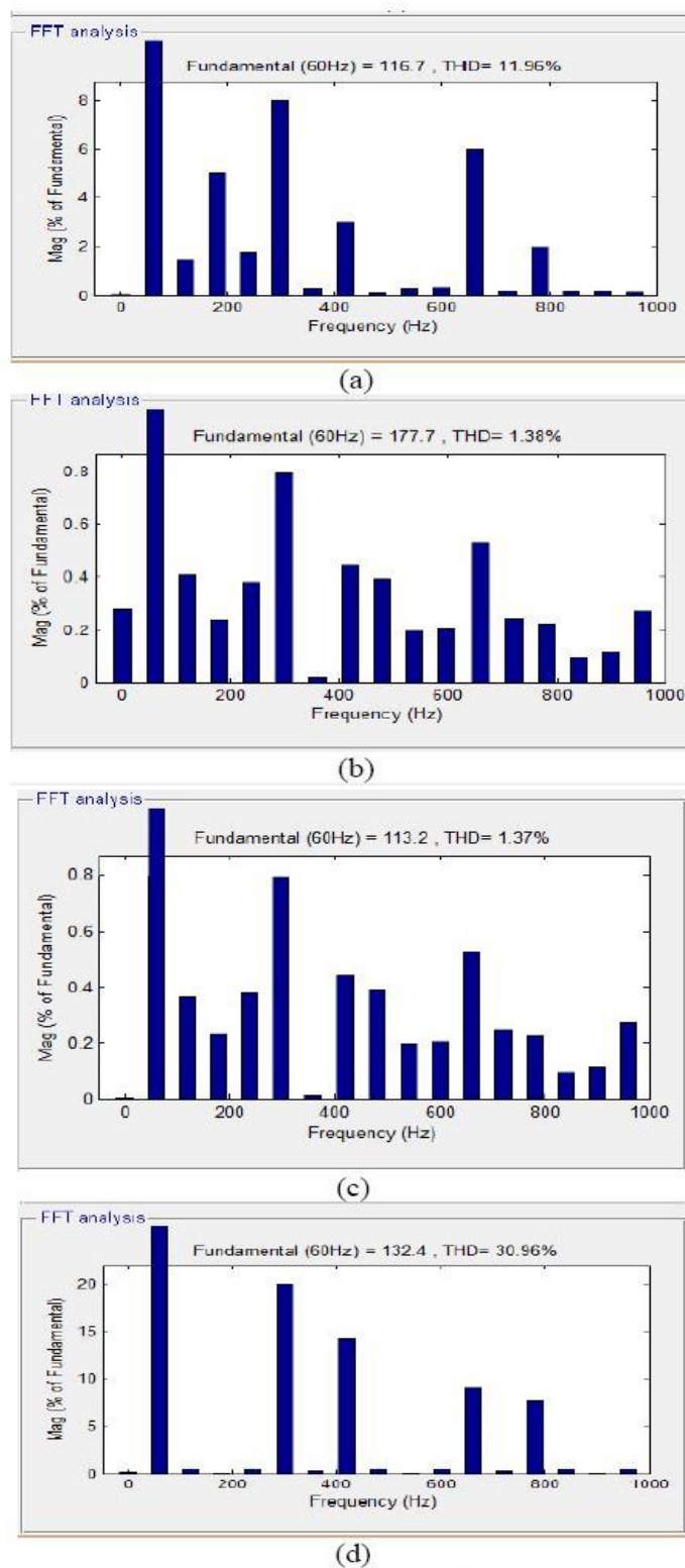
Figure 19: THD while utility receives power. (a) dq-current mode. (b) PV-APF mode. (c) APF mode. (d) Only utility supplies load.
