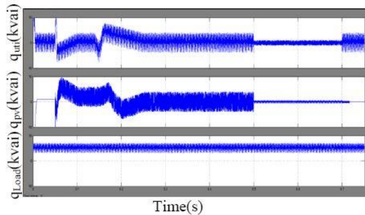
Figure 21: Imaginary power from the (a) utility, (b) PV unit, and (c) load, while the utility receives power.
