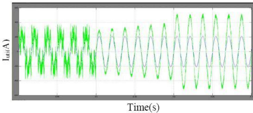
Figure 13: Utility supplied current and PCC voltage waveform.
