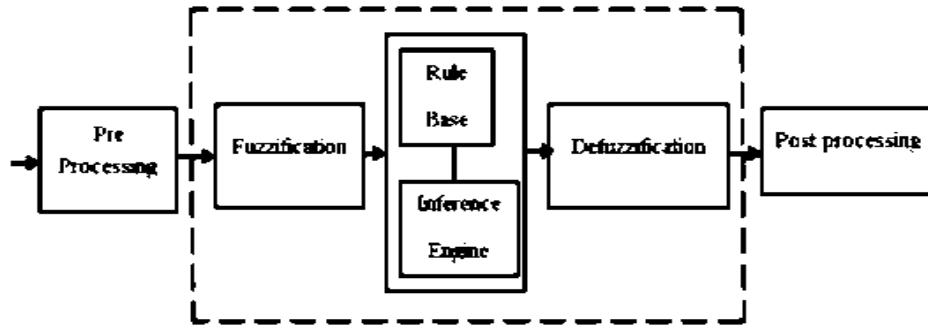
Figure 6: Fuzzy logic controller
