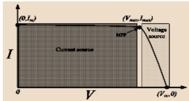
Figure 3: I–V curve and remarkable points.
