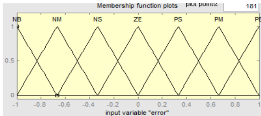
Figure 7: Membership functions
