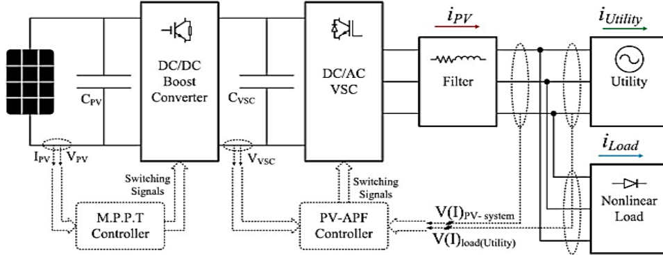
Figure 1: Proposed design of PV-APF combination.
