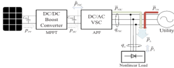
Figure 5: Instantaneous power flows among the PV-APF system.
