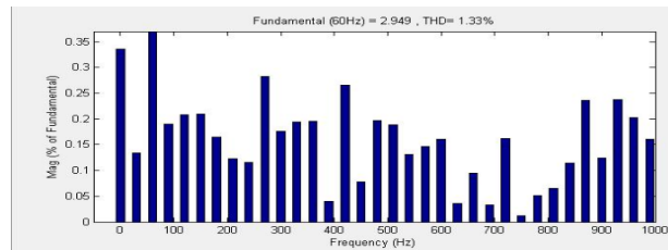
Fig.12.TH D analysis of grid current in PV decreases suddenly mode of operation with PI controller
