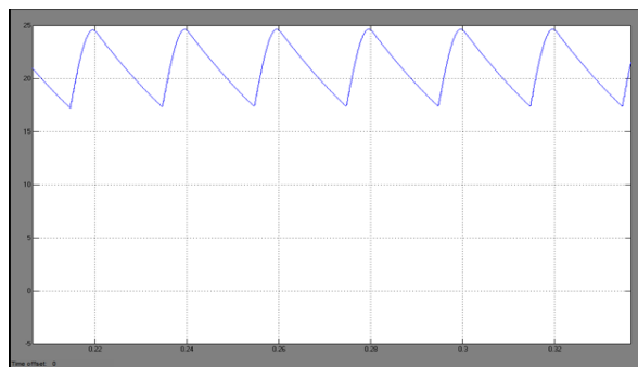
I_{Ln2}
