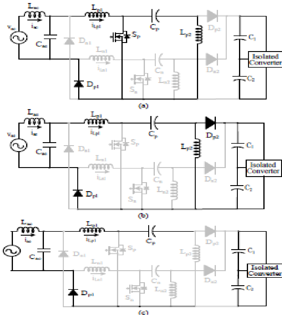
Fig. 3 Operating modes of bridgeless PFC converter when the input voltage is positive
