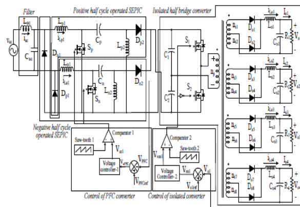
Fig.1 Schematic diagram of the PFC converter based SMPS
