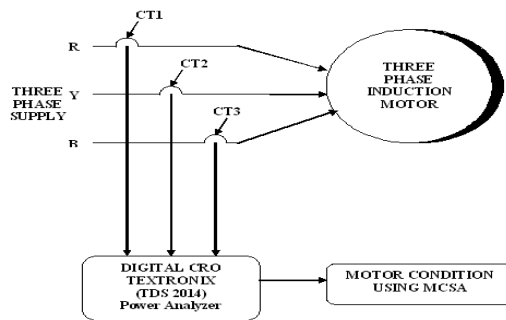
Fig.2. Block diagram of MCSA
