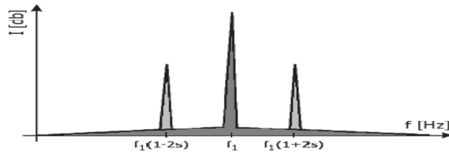
Fig .1. the Idealized current spectrum
