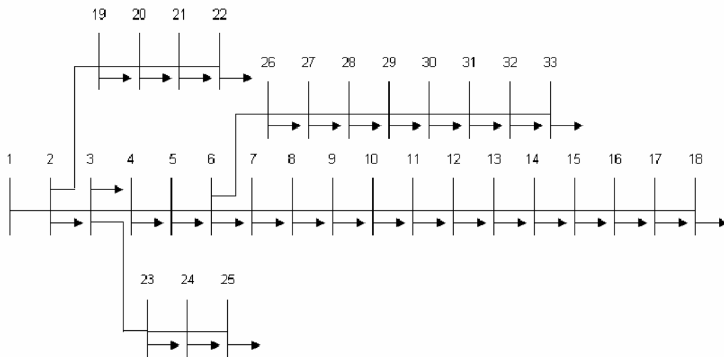
Figure 1: IEEE 33 bus test system.
