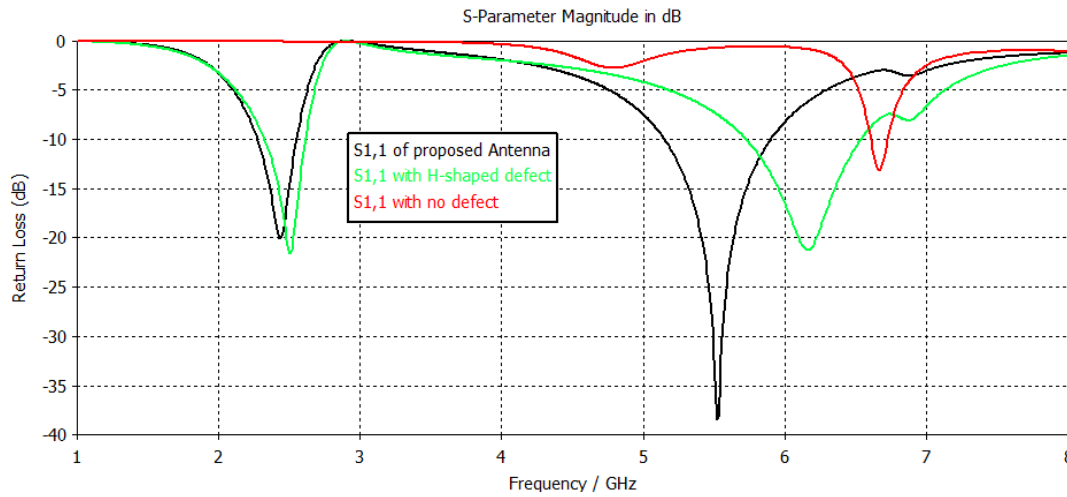
Fig. 2 Simulated Return Loss (dB) against Frequency for Proposed Antenna, with H-shaped and with no Defect
