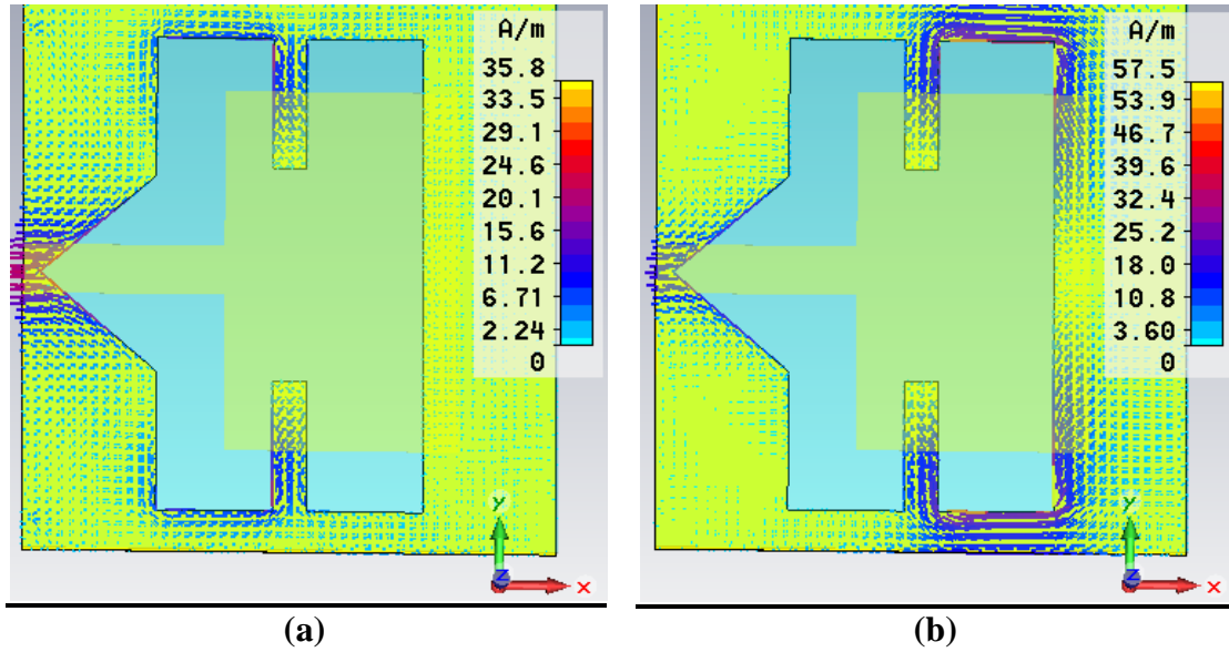
Fig. 4 Surface Current distribution (a) Ground at 2.43 GHz (b) Ground at 5.52 GHz
