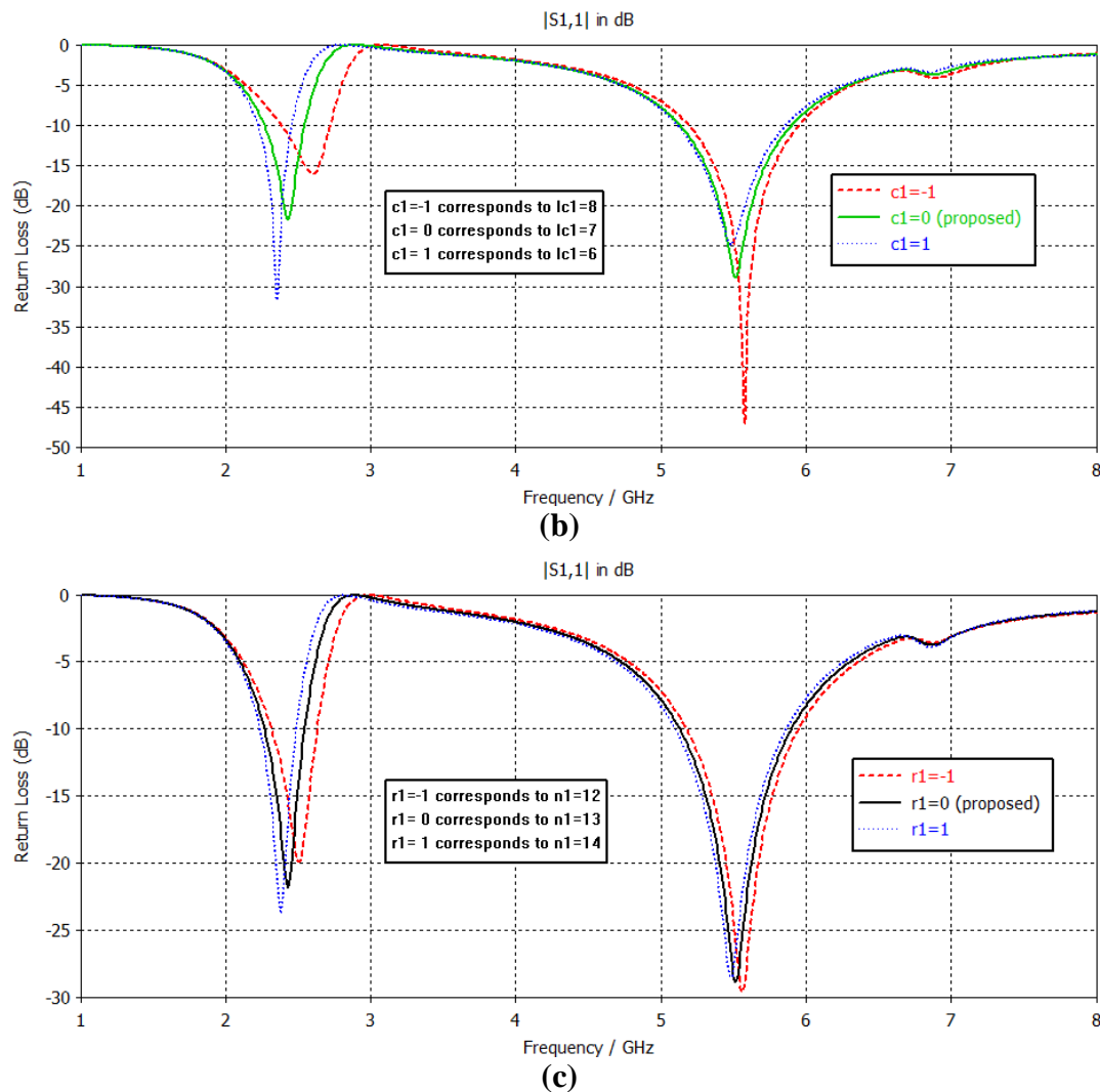
Fig.5 Simulated Return Loss against Frequency for (a) Different values of d_1 (b) Different values of c_1 (c) Different values of r_1
