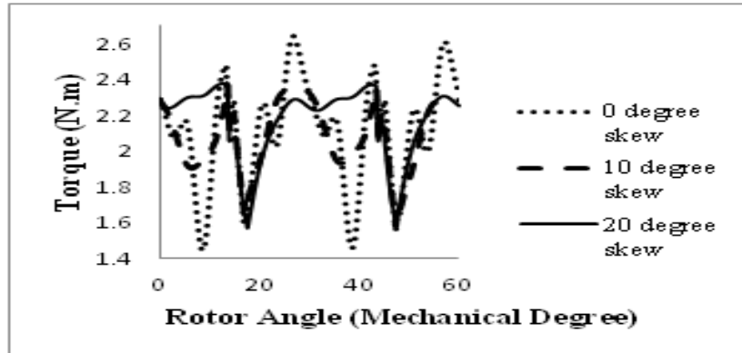
Fig. 4: Torque profiles of designed 200 W radial flux surface mounted PMLDC motor with skewing in rotor poles.
