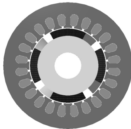
Fig. 3: 20° Skewing in 200 W radial flux PMBLDC motor.
