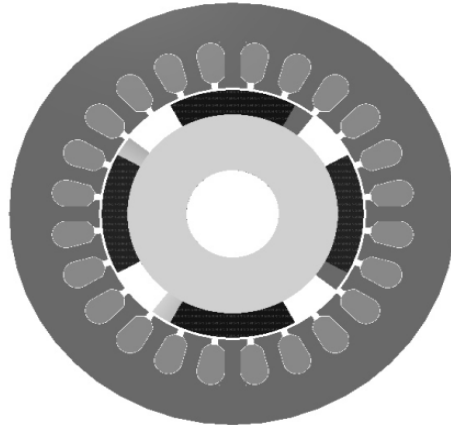
Fig. 2: 10° Skewing in 200 W radial flux PMBLDC motor.
