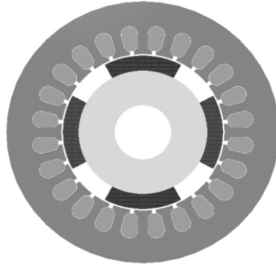
Fig. 1: 0° Skewing in 200 W radial flux PMBLDC motor.
