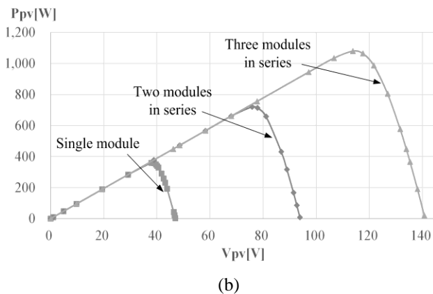
Figure 4. Simulation of a string PV modules without shading condition. (a) Voltage-current characteristics of three different PV module connections, (b) Voltage-power characteristics of three different PV module connections.
