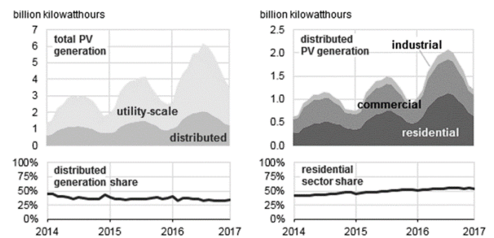
Figure 1. U.S. electricity generation from solar PV systems, according to U.S. Energy Information Administration, Electric Power Monthly.
