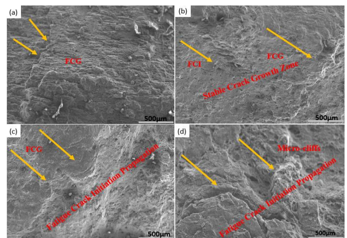
Figure 8: Fatigue fracture Morphology of cavitation water jet peening at different pressures (a) unpeened, (b) 20 MPa, (c) 25MPa, and (d) 30MPa.
