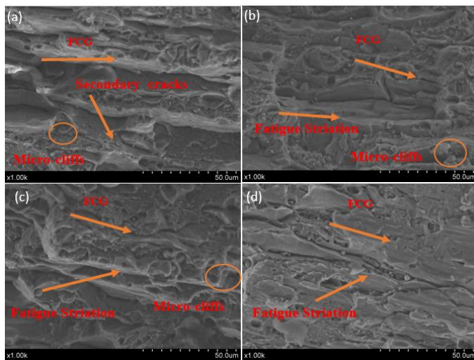
Figure 9: Fatigue striation of different pressures of cavitation water jet peening. (a) Unpeened (b) 20MPa, (c) 25MPa and (d) 30MPa.
