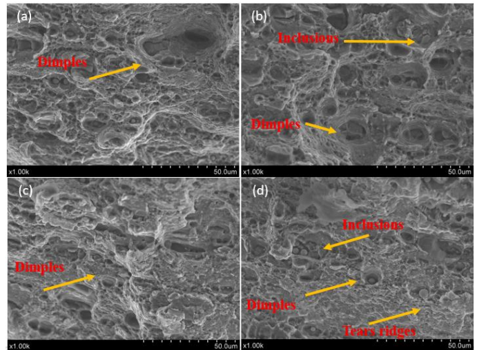
Figure 10: Fracture Morphology of Dimples Coalescence Different Pressures of Cavitation Water Jet Peening. (a) Unpeened (b) 20MPa, (c) 25MPa and (d) 30MPa.
