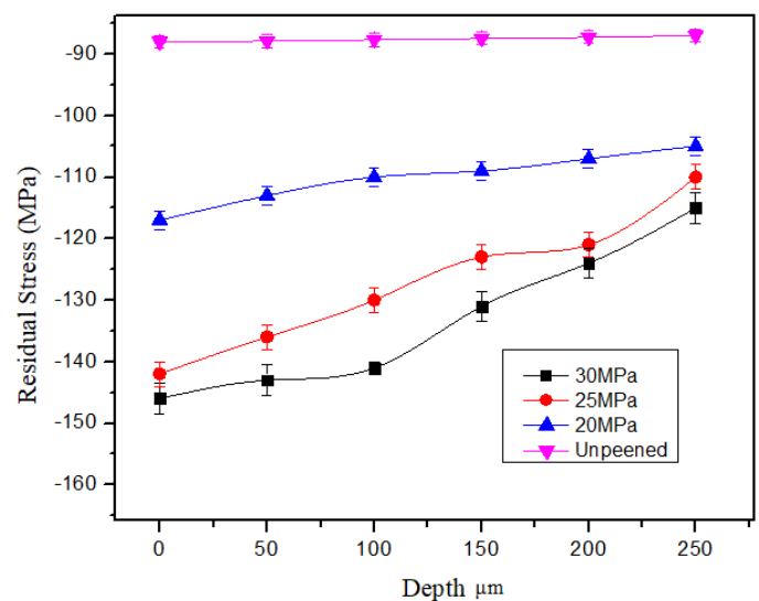
Figure 6: Distribution of residual stress field of 8090 aluminium alloy lithium with different pressure.
