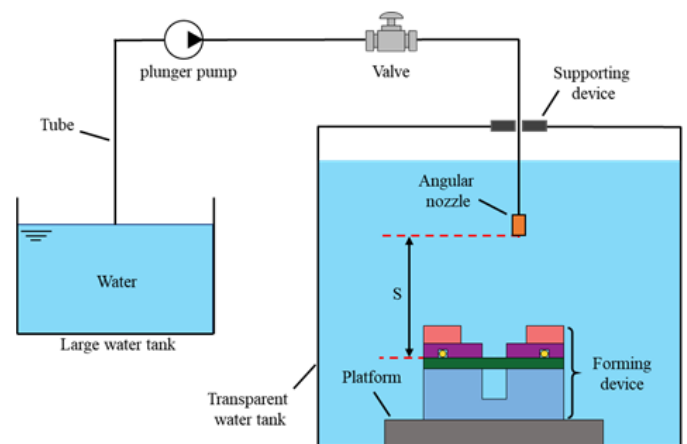
Figure 1(a): Water-jet cavitation experimental system.
