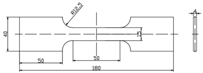
Figure 1: Fatigue test sample and parameters (unit: mm).
