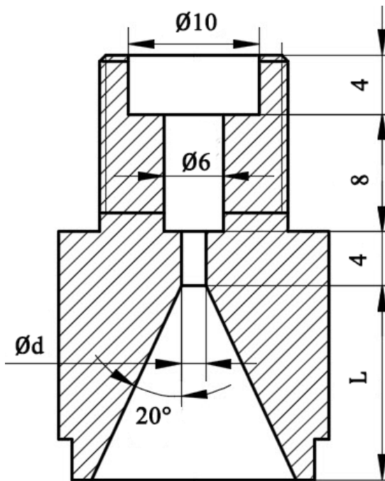
Figure 2: Nozzle geometry diagram.
