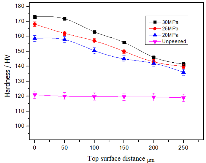
Figure 5: Vickers hardness curves of 8090 aluminum-lithium alloy with different peening pressure.
