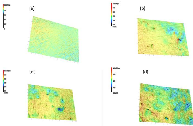
Figure 4i: 3D surface contour roughness; (a) Unpeened, (b) 20MPa, (c) 25MPa, and (d) 30MPa.
