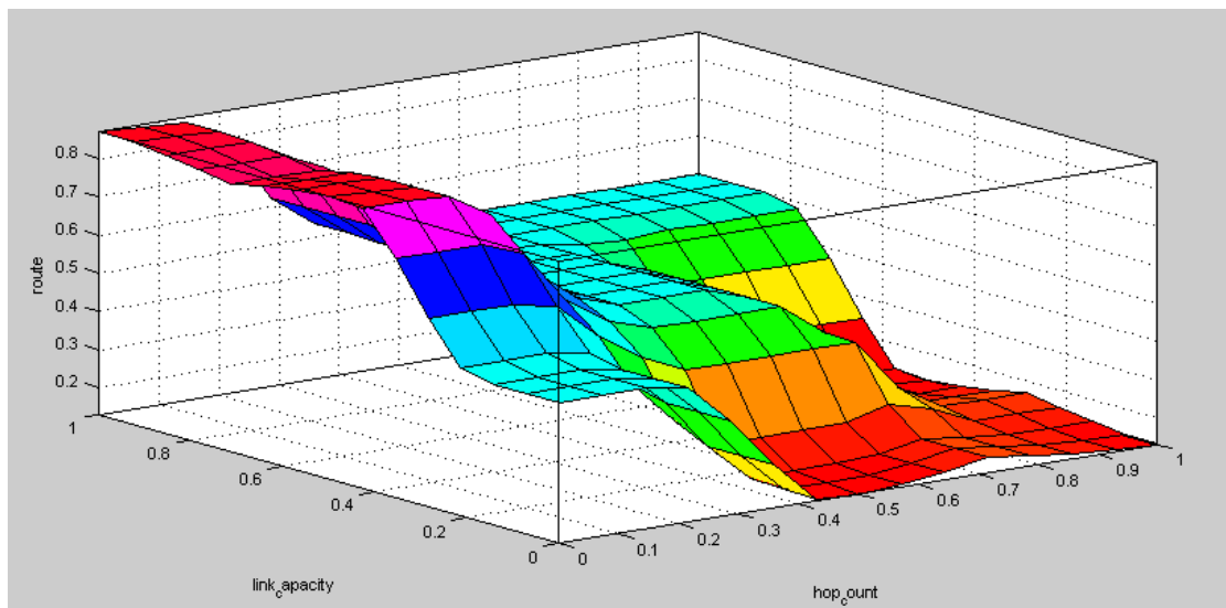
Fig.5: 'Route' O/P w.r.t. 'Hop Count' and 'Link Capacity'
