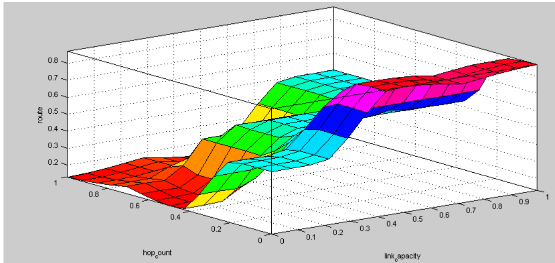
Fig.6: 'Route' O/P w.r.t. 'Link Capacity' and 'Hop Count'
