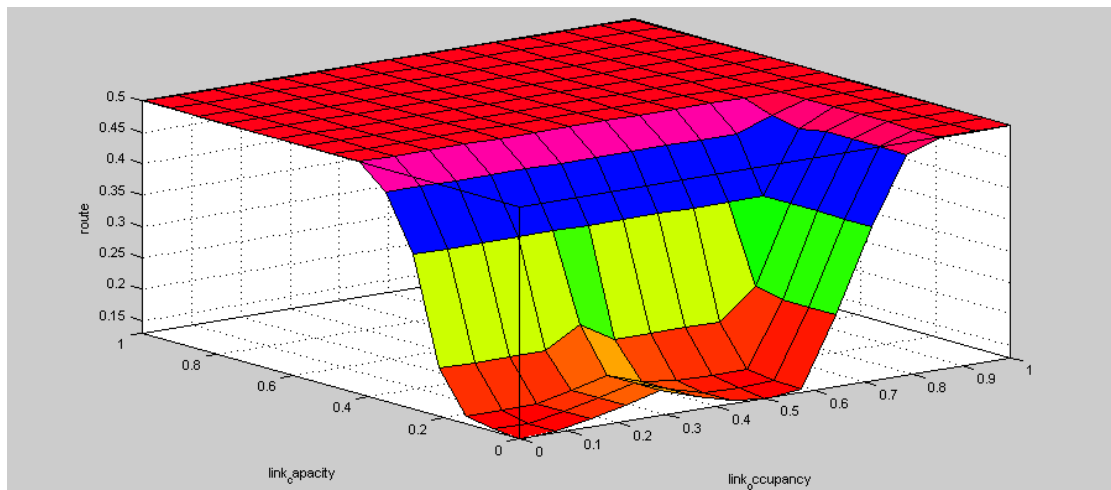
Fig.3: ‘Route’ O/P w.r.t. ‘Link Capacity’ and ‘Link Occupancy’
