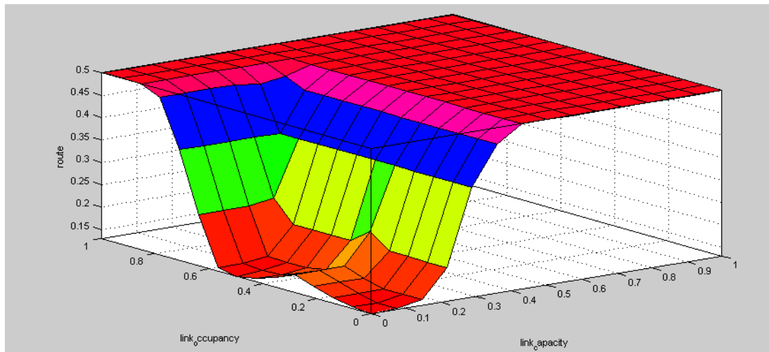
Fig.4: 'Route' O/P w.r.t. 'Link Occupancy' and 'Link Capacity'
