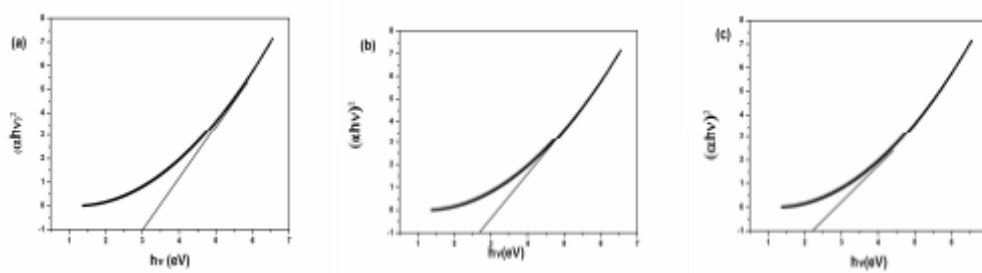
Figure 6: Tauc plots of (a) as prepared CuO nanoparticles, (b) CuO nanoparticles annealed at 300 °C, (c) CuO nanoparticles annealed at 600 °C
