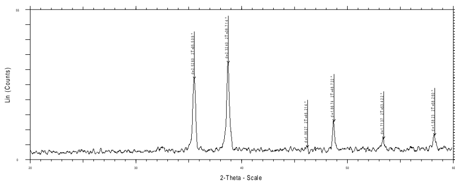
Figure 4: XRD pattern of the as prepared CuO nanoparticle annealed at 600°C
