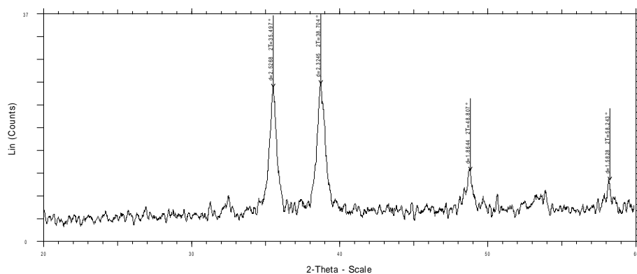
Figure 3: XRD pattern of the as prepared CuO nanoparticle annealed at 300°C
