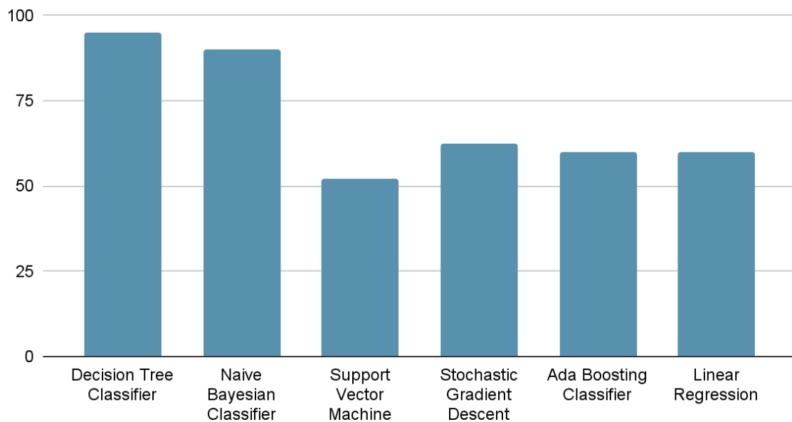
Figure 5: Comparison of accuracies of the machine learning models.
